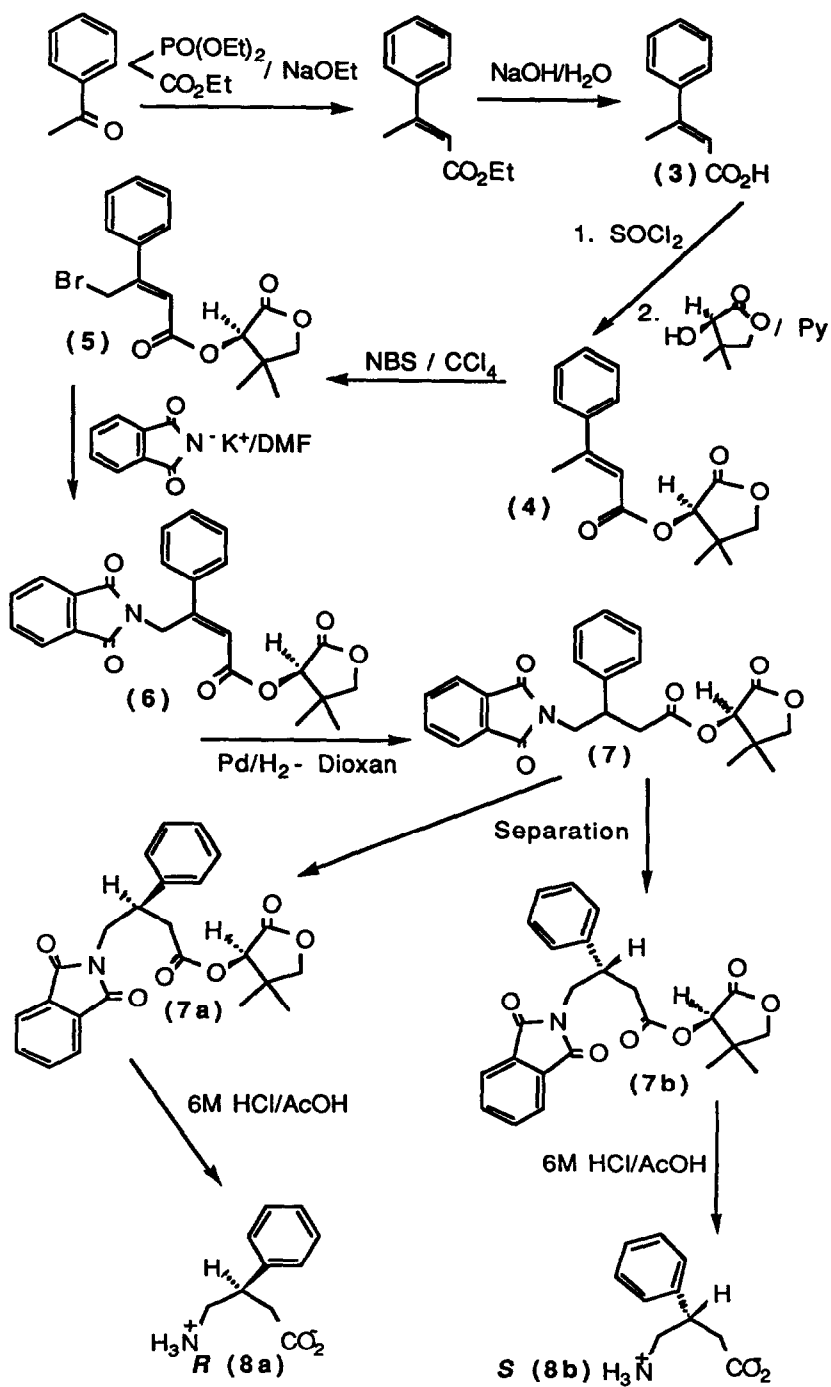
Scheme 1
